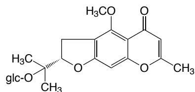
4'-O-Glucosyl-5-O-methyl visamminol (ボウフウ)
