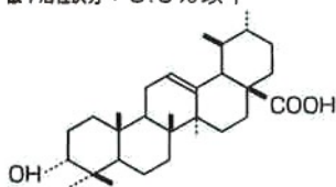
ursolic acid
